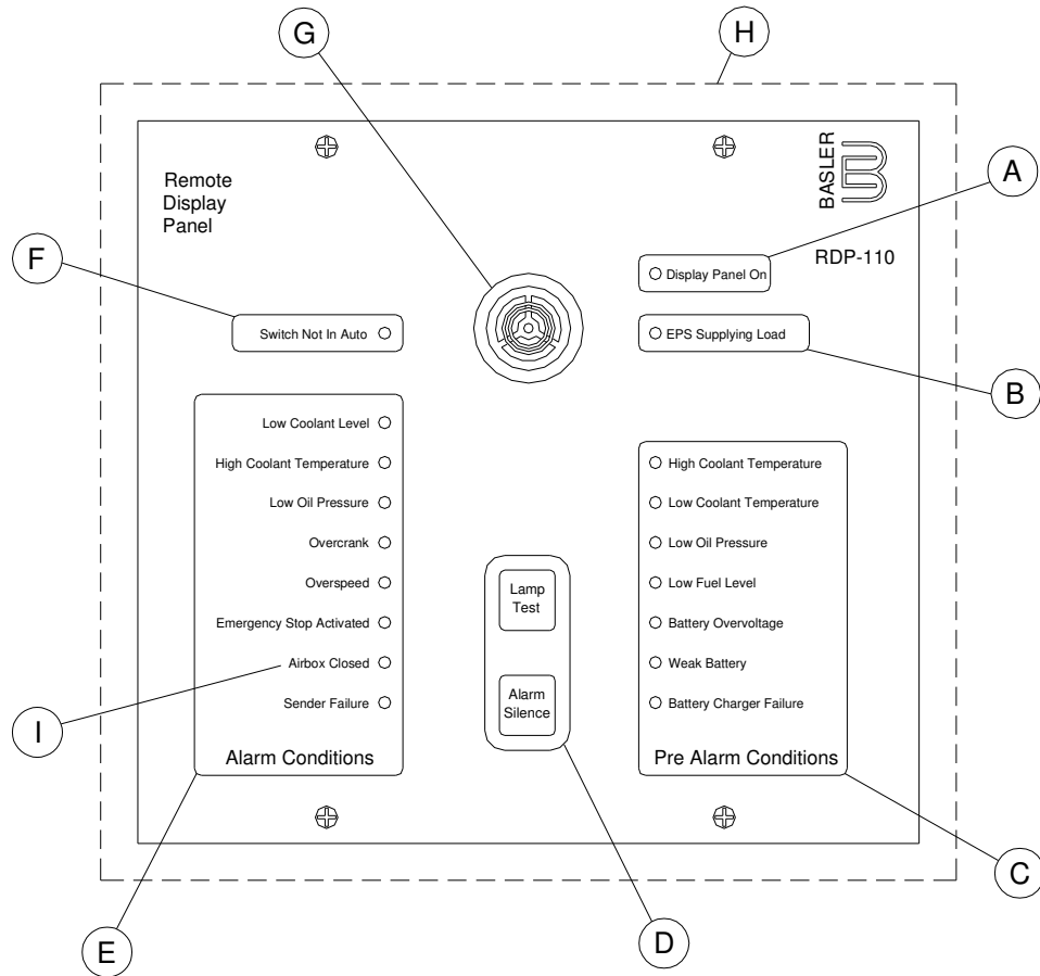
Figure 2 – Front panel controls and indicators
