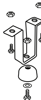
FIGURE 7: Rubber Stopper Attachment to Support Leg
