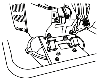
FIGURE 28: Oil Drain Bolt
