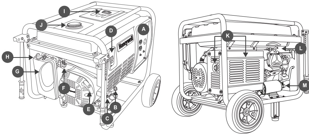
FIGURE 16: HW6200L Portable Generator
